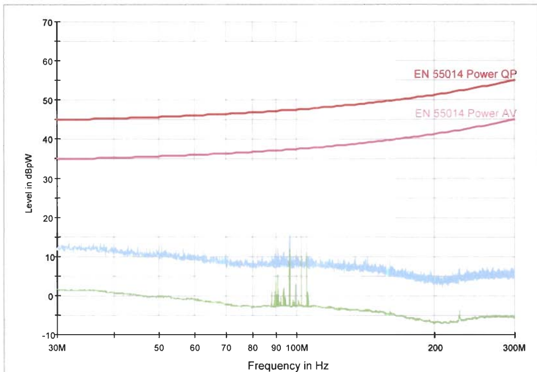
EN55014 Power
