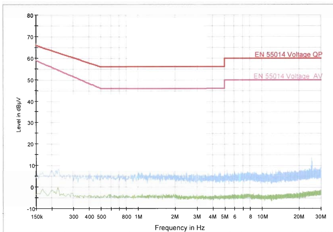
EN55014Voltage
